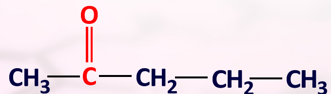
2-pentanon
