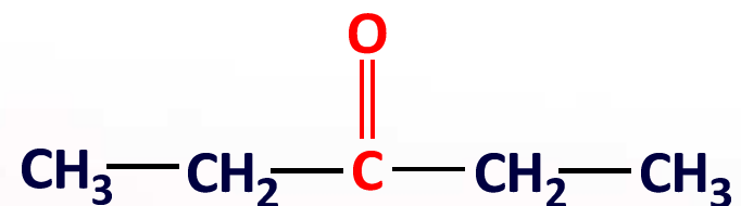
3-pentanon
