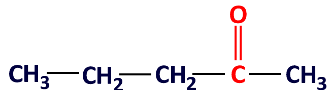
2-pentanon
